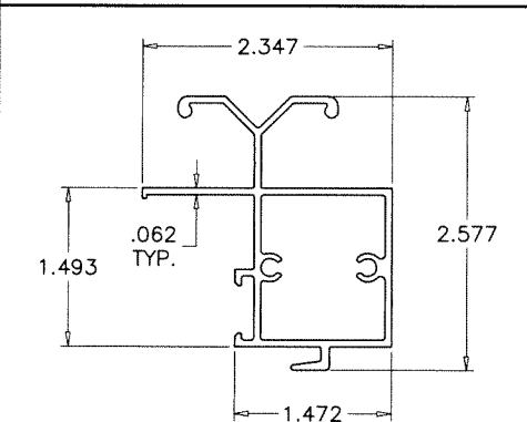
⑦ VENT INTERLOCK W/ HANDLE
