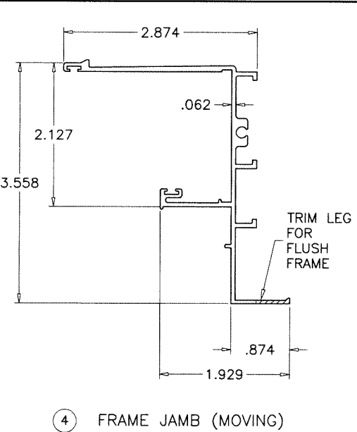
③ FRAME JAMB (MOVING/FIXED)
